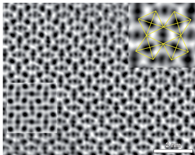
Figure 3. ABF-STEM image of \zeta - \text{Mn}_2\text{O}_3 taken along the \langle 100 \rangle_p perovskite direction. Inset: projections of the corner-sharing in-phase tilted \text{MnO}_6 octahedra (yellow lines). The dots between the octahedra indicate the projections of the Mn atomic columns at the perovskite A-sites. The inserted calculated [001] ABF-STEM image (white box) was obtained with the atomic coordinates of \zeta - \text{Mn}_2\text{O}_3 (Table S10) at a thickness t = 79 Å.
